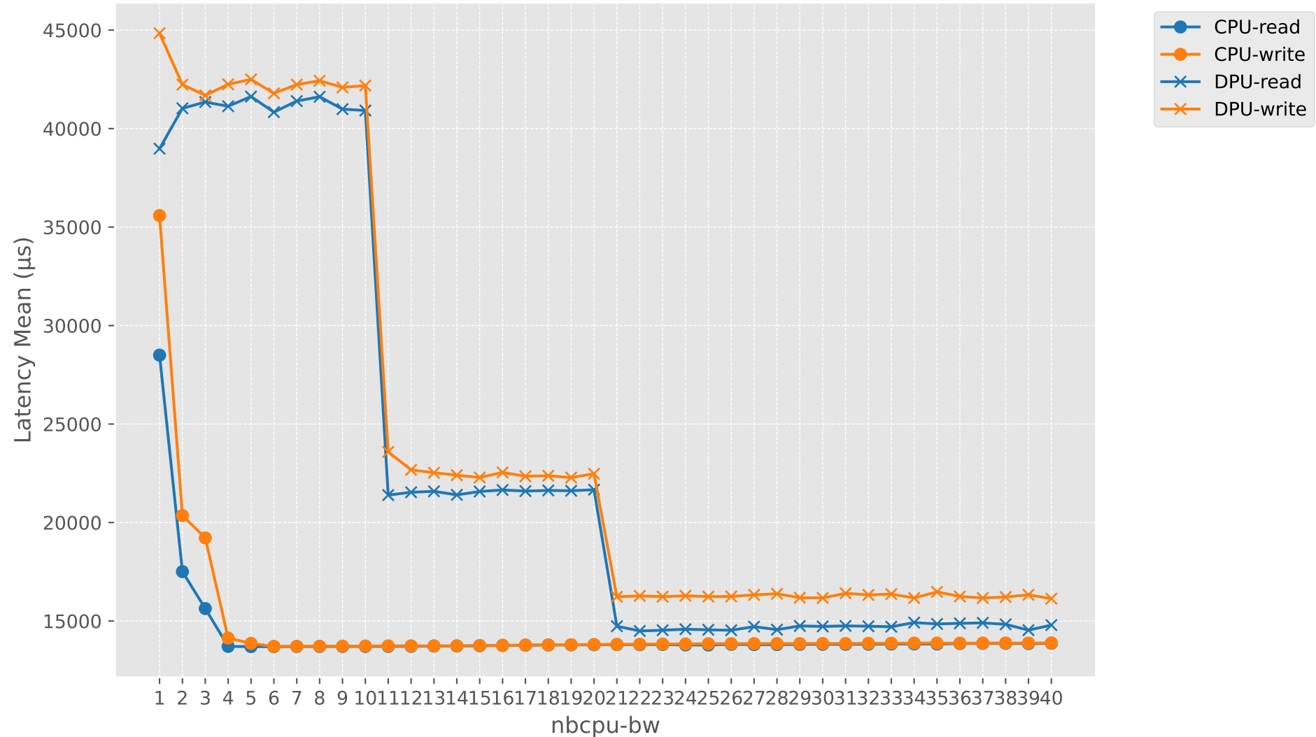
Latency Mean vs nbcpu-bw (CPU vs DPU)
